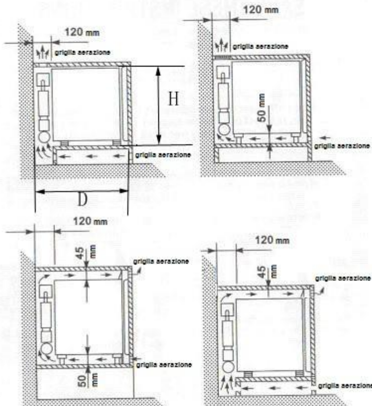
Installation Figure (side view of the refrigerator)
